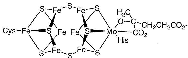
Figure 8.2 Structure of Fe-Mo cofactor in nitrogenase.
